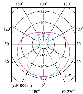
Light Distribution Diagram - CorePro LEDtube 1200mm 16W 865 T8 AP I
