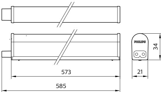
BN068C LED6/CW L600 G2
